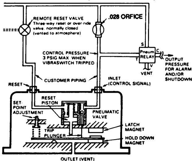
PIPING DIAGRAM - MODEL 368
