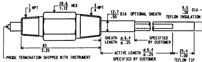
INSULATED PROBE
